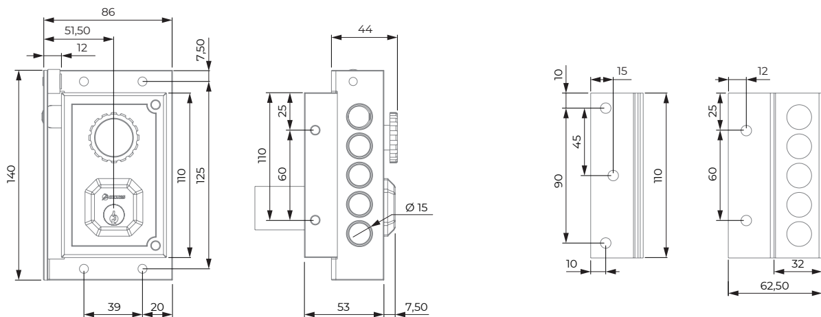
CONTRAPLACA COUNTERPLATE
