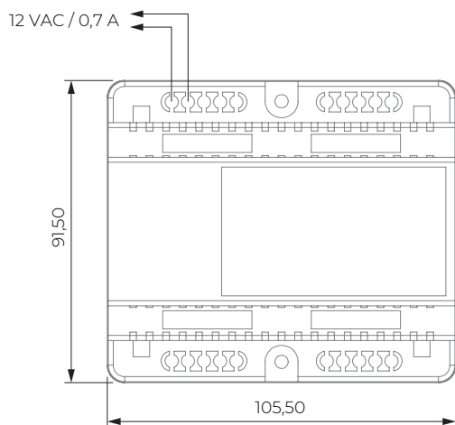
MÓDULO RECEPTOR RECEIVER MODULE
